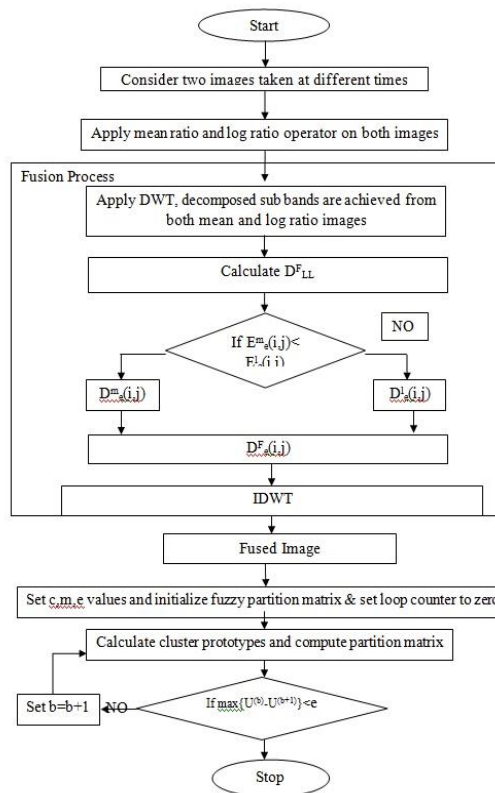
Fig.1. Flowchart of the proposed change detection approach
